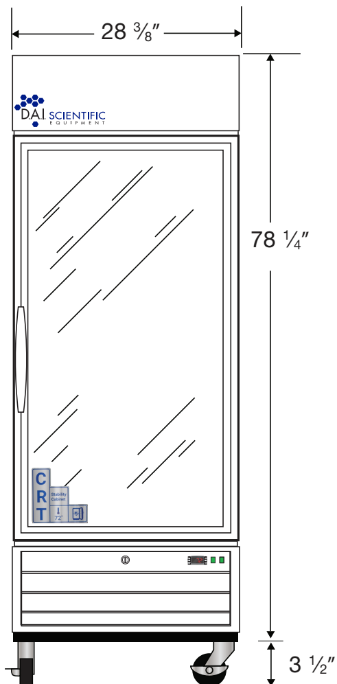
Front View
