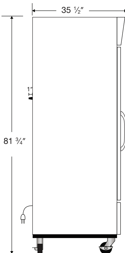
Side View
