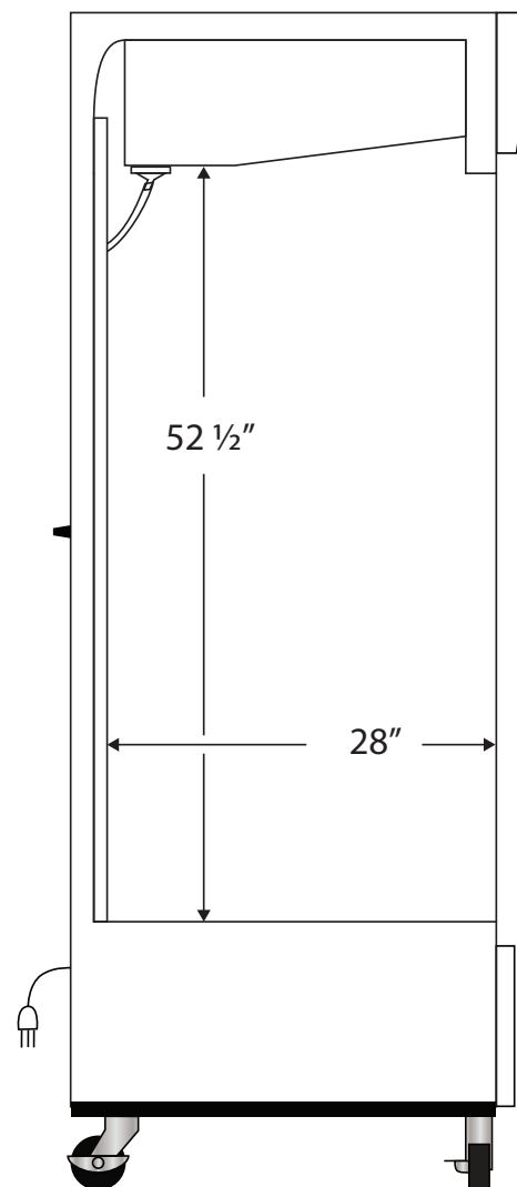
Side View
