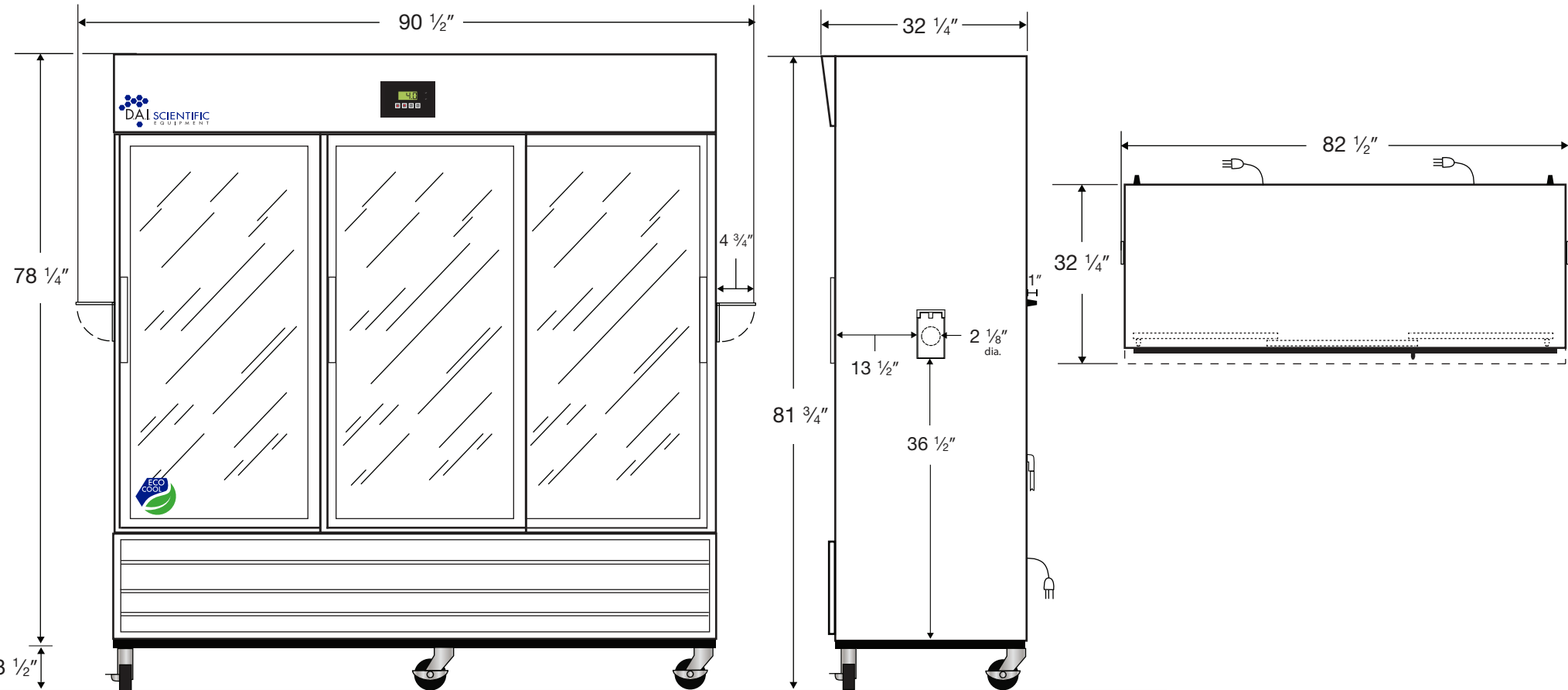
Top View
