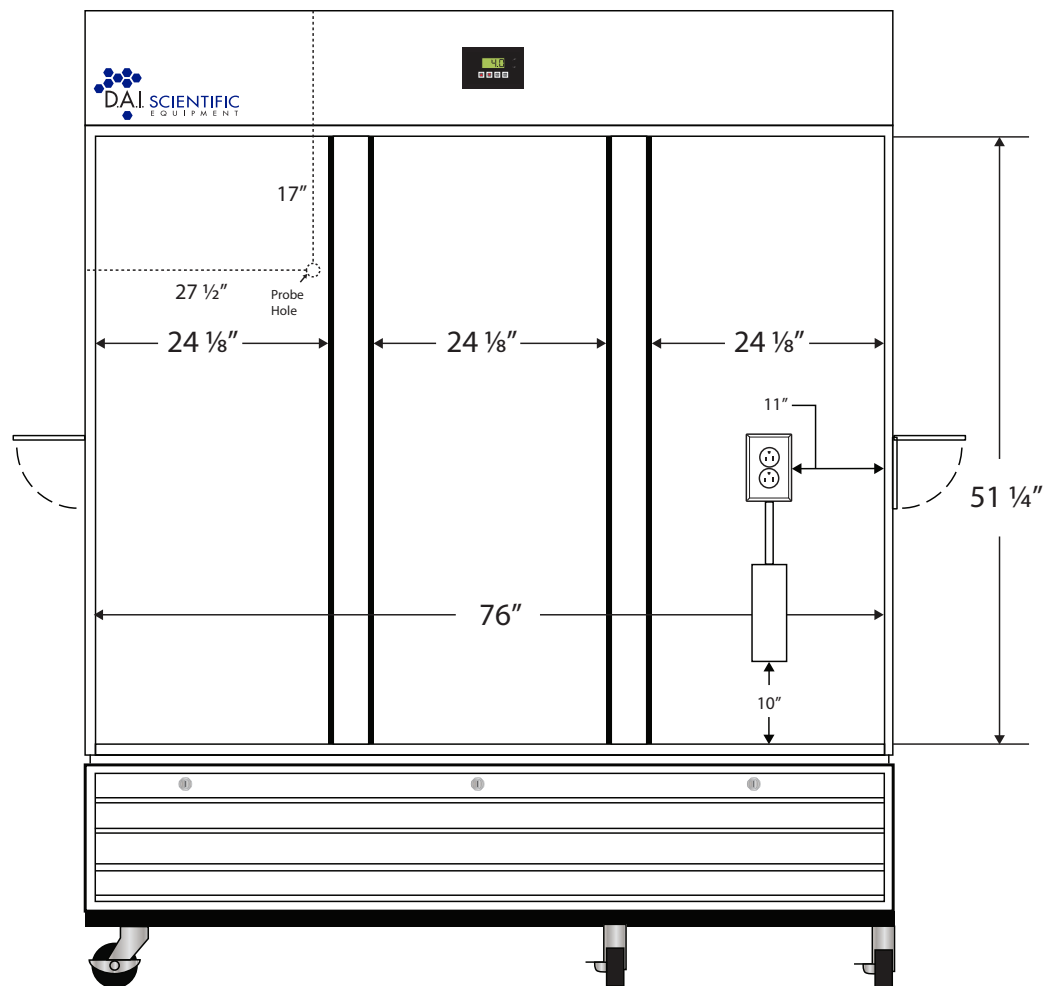
Front View
